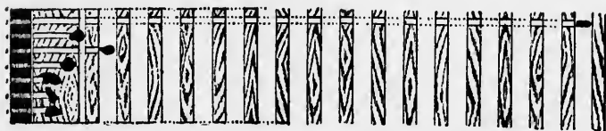
3. Compound. 4, 5, 6. Hard lead bullets. 7, 8, 9. Soft bullets.
